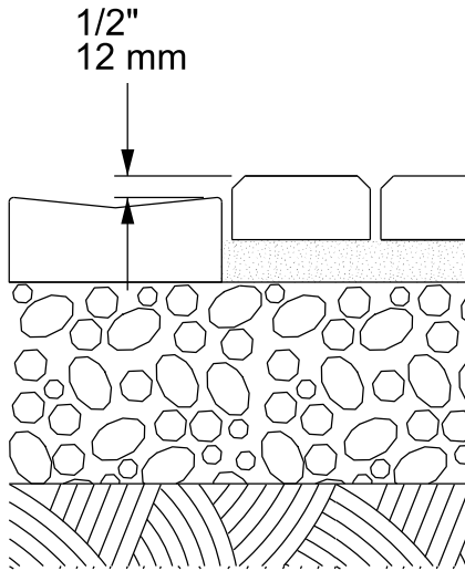
GUTTER
